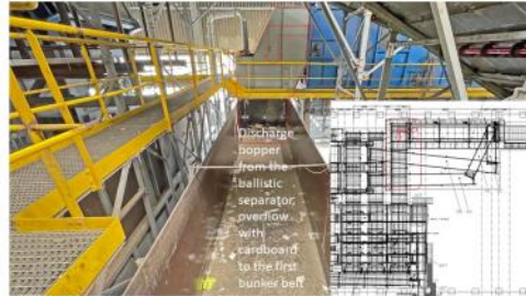
Overflow (cardboard) from the ballistic separator
